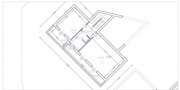
PIANO INTERRATO
